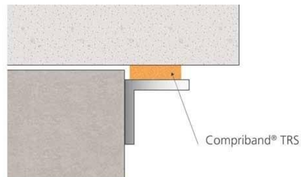
Croquis : Joint solin
